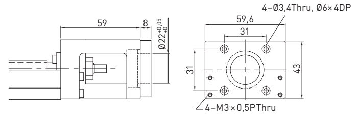
Motor adapter flange F7
