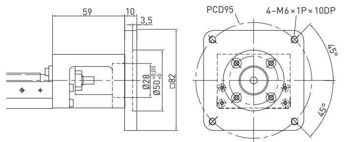
Motor adapter flange F11
