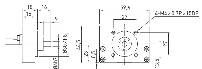
Motor adapter flange H1
