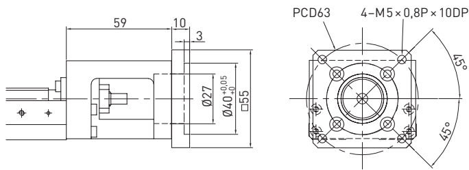
Motor adapter flange F6
