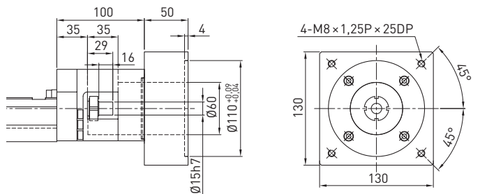
Motor adapter flange F5
